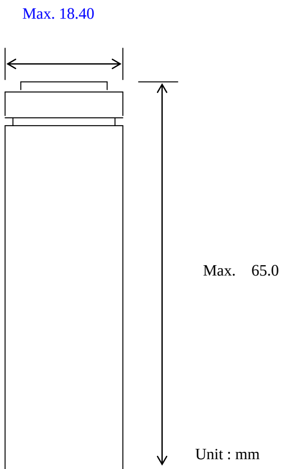
Fig.1. Outline Dimensions of ICR18650-32A
