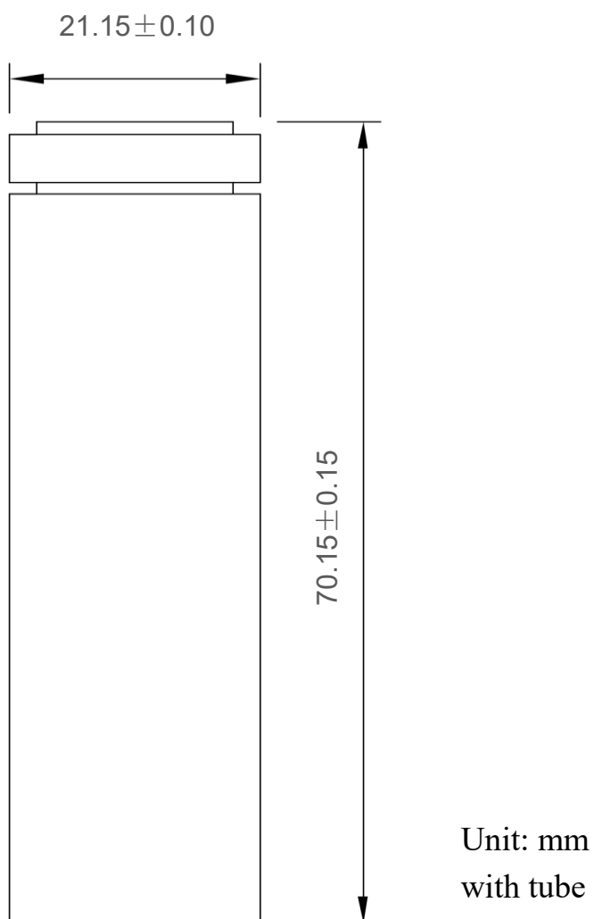
Fig. 1. Outline Dimensions of INR21700/40PL
