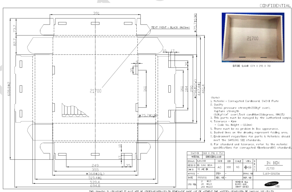
Fig. 2-2. Inner box package drawing.
