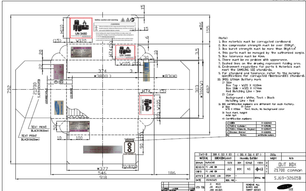
Fig. 2-1. Outer box package drawing.
