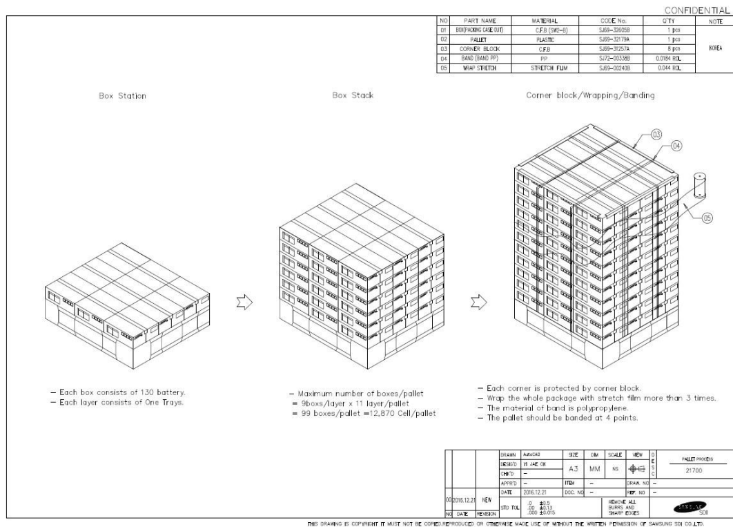
Fig. 2-5. Pallet packaging process
