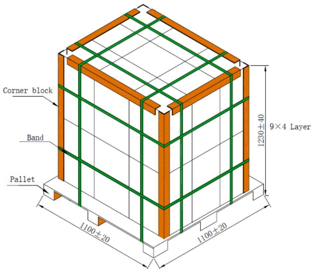
Fig. 4.Air transportation package
